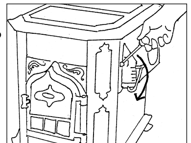
To engage to catalytic combustor, simply push up the bypass handle
