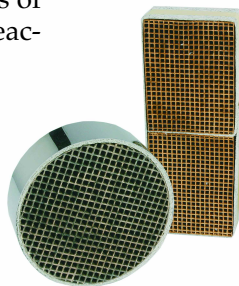
A catalytic combustor is a ceramic honeycomb coated with precious metals
